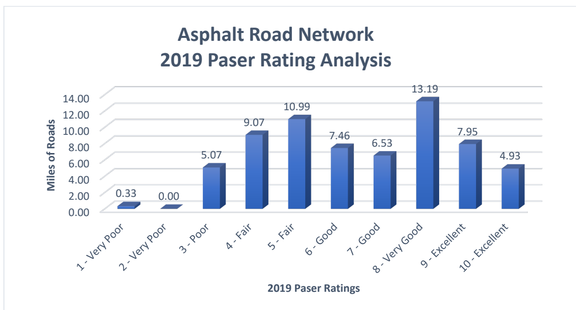
FIGURE 1A: Asphalt Road Network 2019 PASER Rating Analysis
